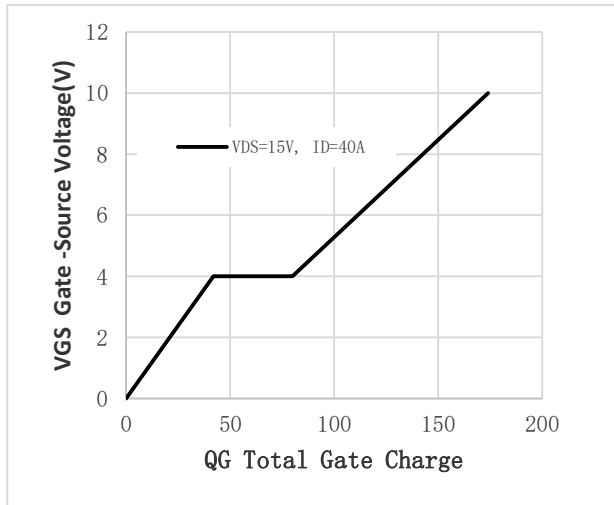
Fig.1 Gate-Charge Characteristics
