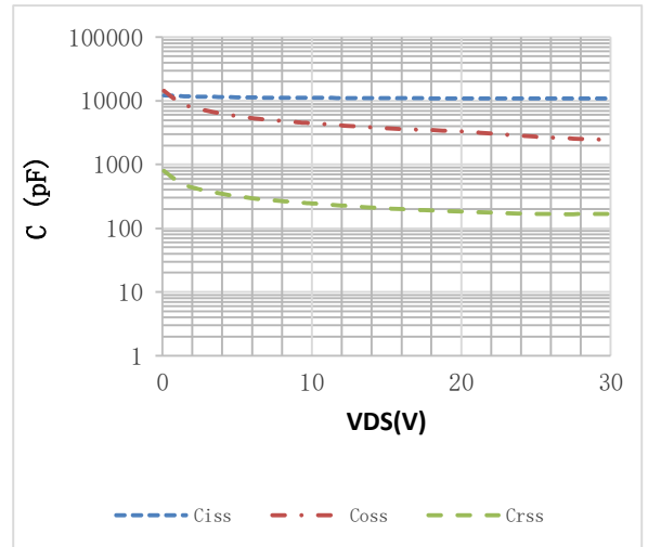
Fig.2 Capacitance Characteristics
